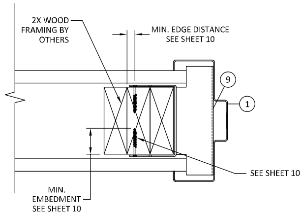
G 7 HORIZONTAL SECTION COMBINATION ANCHOR WOOD STUD
