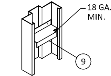
DETAIL CC Z ANCHOR
