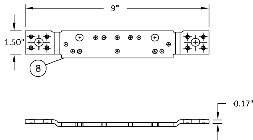
DETAIL KK FRAME HINGE REINFORCEMENT
