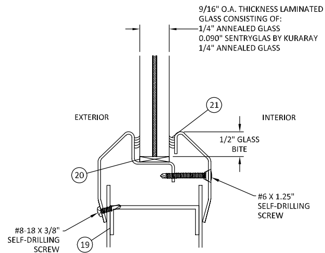
GLAZING DETAIL
