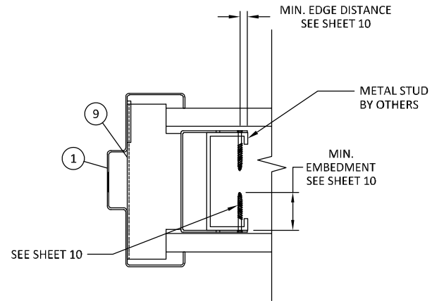
H 7 HORIZONTAL SECTION COMBINATION ANCHOR METAL STUD
