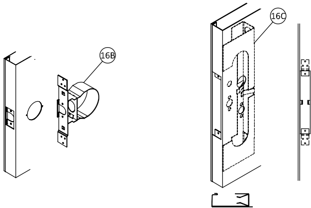
DETAIL OO CYLINDRICAL LOCK REINFORCEMENT
